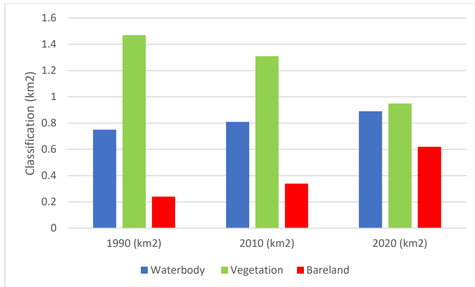
Fig. 6. Land use change from 1990 to 2010 and 2020.
