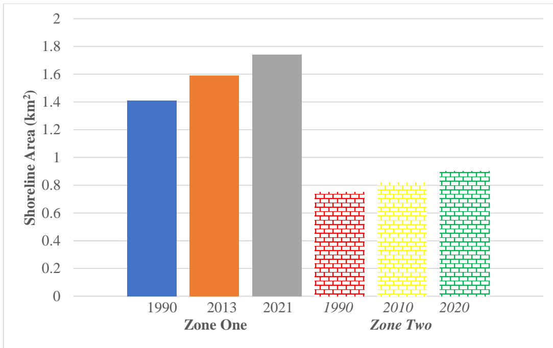
Fig. 9. Shoreline changes from 1990 to 2021
