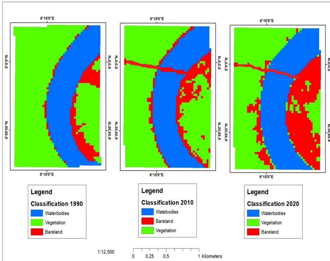
Fig. 5. Land use classification of zone two for 1990, 2010, and 2020.
