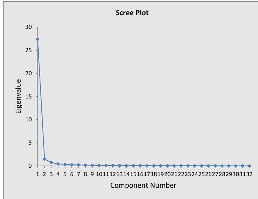
Fig. 1 Scree Plot
