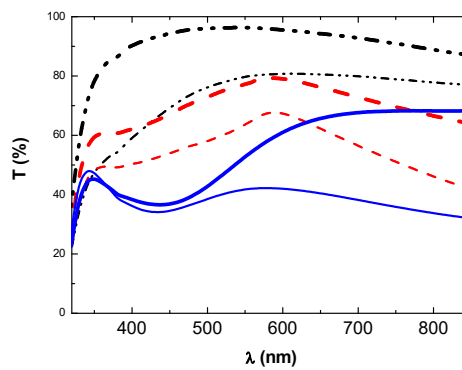
Figure 15: Colour change induced by polarization inversion in different EC-devices : (- - - - -) ITO//ITO, (- - - - -) \text{WO}_3 / \text{Ag} / \text{Cu} : \text{Al} / \text{WO}_3 // \text{ITO} and (—) \text{WO}_3 / \text{Ag} / \text{Cu} : \text{Al} / \text{Pt} / \text{WO}_3 // \text{ITO} .
