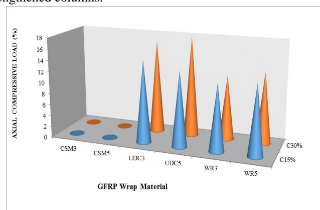
Figure 7. Effect of GFRP Wrap Material on Load Carrying Capacity of Corrosion-Damaged Columns
