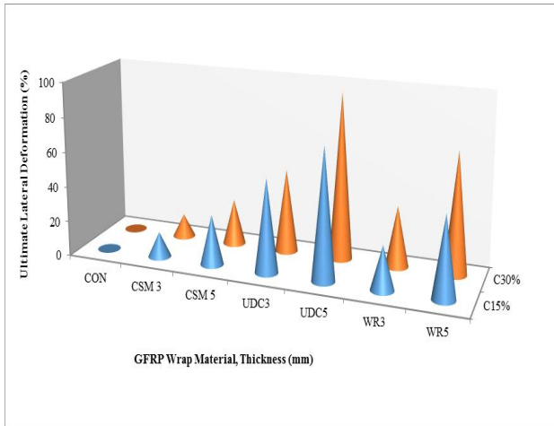
Figure 10. Effect of Various Levels of Corrosion-Damage on Lateral Deformation of GFRP Wrapped Columns
