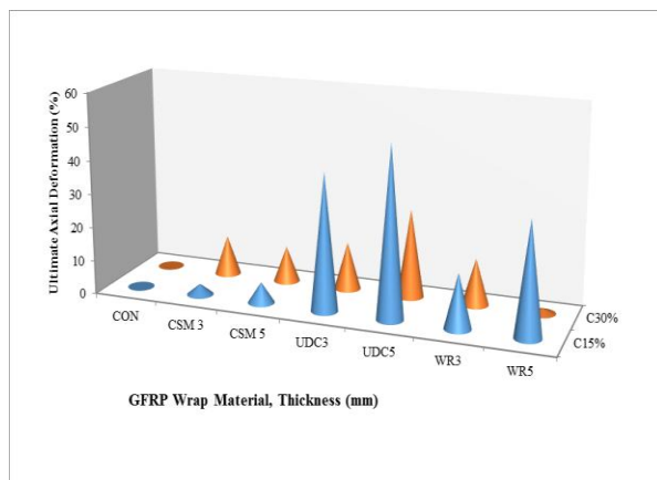
Figure 8. Effect of Various Levels of Corrosion-Damage on Axial Deformation of GFRP Wrapped Columns
