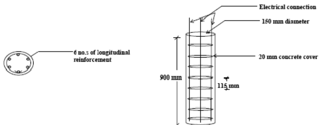
Figure 4: Column Details
