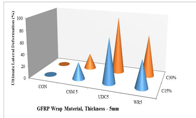
Figure 13. Effect of 5 mm Thick GFRP Wrap on Lateral Deformation of Corrosion-Damaged Columns
