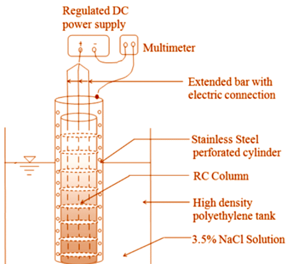
Figure.5: Schematic View of Accelerated Corrosion Set-up
