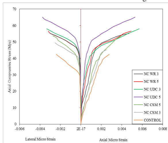
Figure 14. Stress-Strain Response for 0% Level of Corrosion-Damaged Columns
