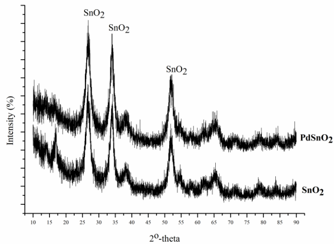
Figure 6: XRD diffractogram of SnO 2 and PdSnO 2
