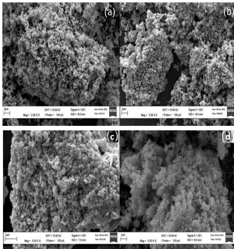
Figure 7: SEM micrograph for (a) Pd/ZnO (wet-impregnation), (b) Pd/ZnO (sol-gel), (c) SnO 2 and (d) PdSnO 2
