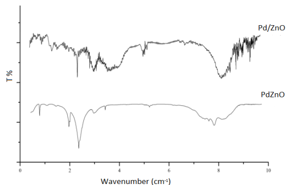
Figure 9: FTIR spectra of PdZnO (wet-impregnation) and Pd/ZnO (sol-gel)
