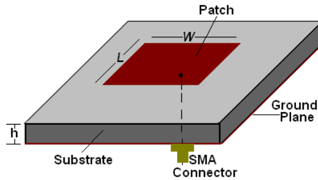
Figure 1: Microstrip Antenna Configuration
