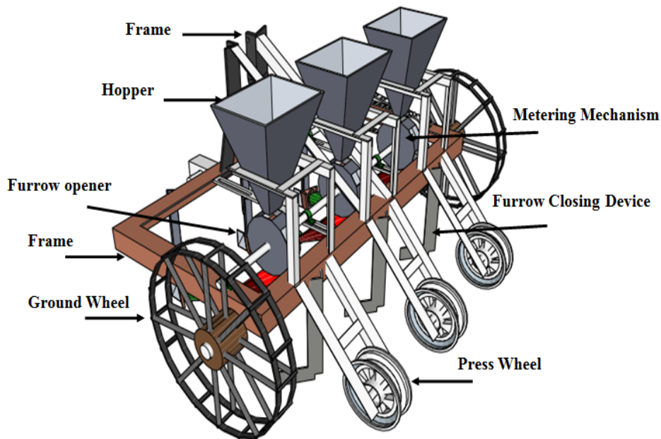
Figure 1: The 3D drawing of the seed planter
